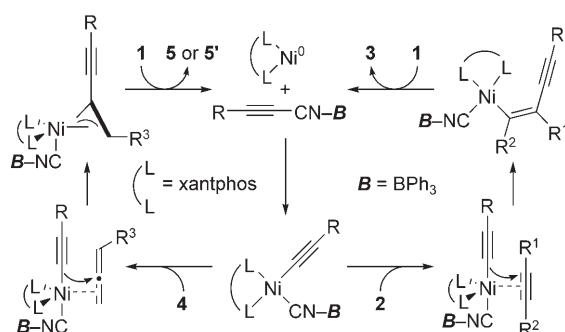
Scheme 1. A plausible mechanism for the nickel/BPh 3 -catalyzed alkynylcyanation.
