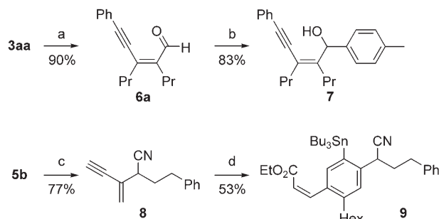
Scheme 2. Transformations of the alkynylcyanation products. a) DIBAL-H, toluene, –78 °C, 2 h, then SiO 2 ; b) p -tolylmagnesium bromide, Et 2 O, 0 °C, 2 h; c) TBAF, AcOH, THF, RT, 1 h; d) (Z)-Hex-C≡C-CH=CH-CO 2 Et, (Bu 3 Sn) 2 O, [Cp(allyl)Pd] (5 mol %), 2-CyN=CH-C 6 H 4 -PPh 2 (10 mol %), THF, 50 °C, 24 h. Cp = cyclohexyl, DIBAL-H = diisobutylaluminum hydride, TBAF = tetrabutylammonium fluoride.
